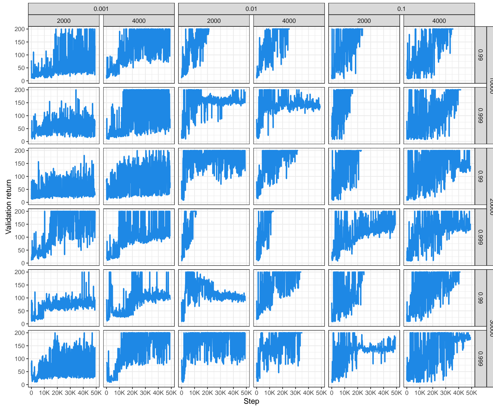
Data Re-Uploading – Skolik et al. – Global Scaling with Pooling (GSP) – Scaled and Continuous (SC)
