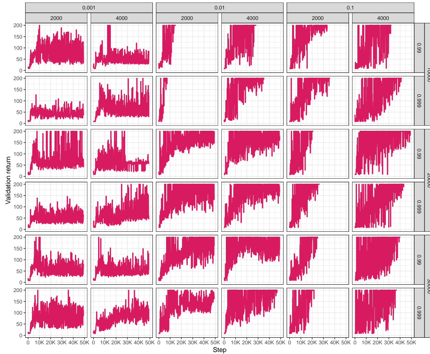
Data Re-Uploading – Skolik et al. – Global Scaling with Pooling (GSP) – Continuous (C)
