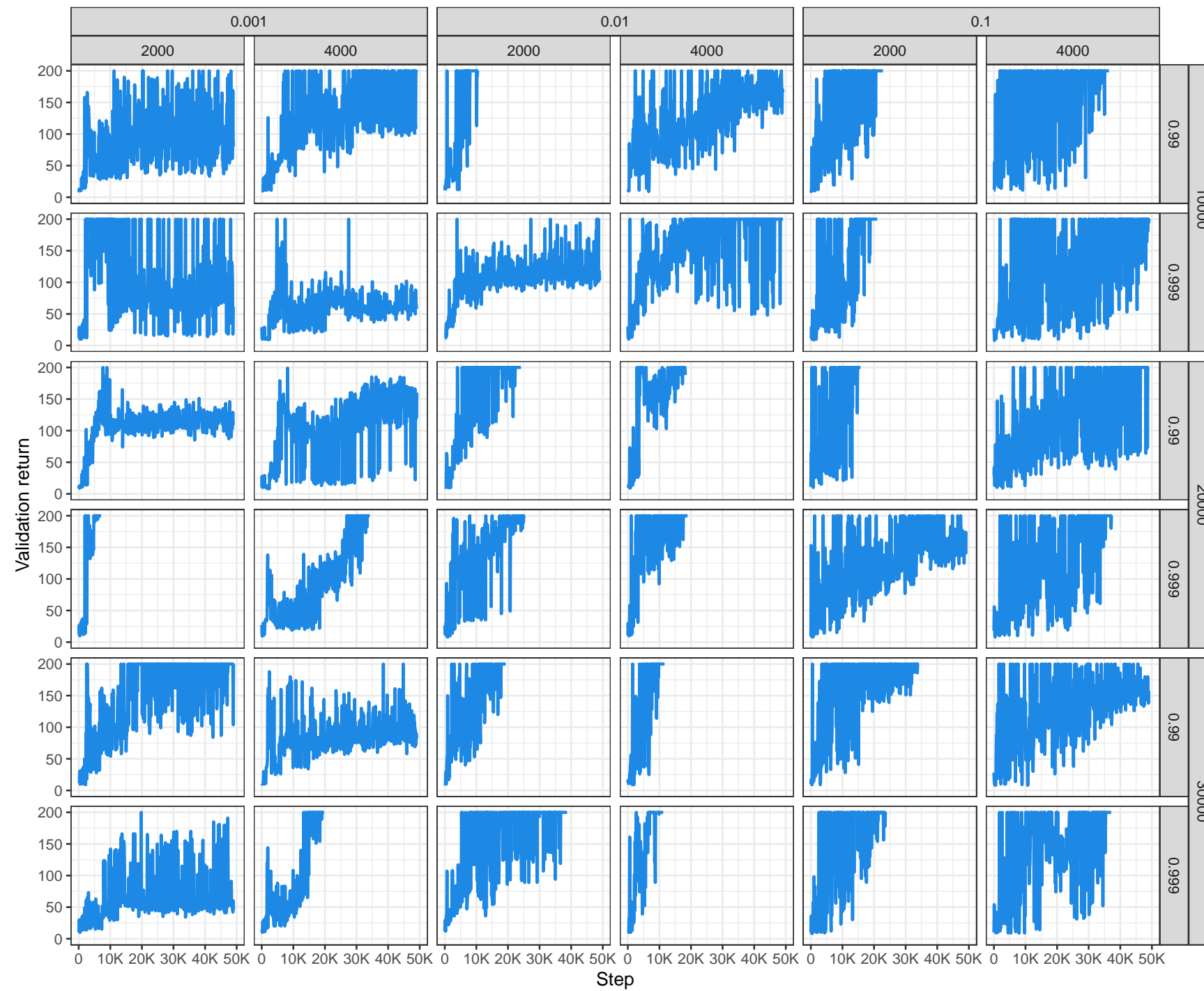
Data Re-Uploading – Skolik et al. – Global Scaling (GS) – Scaled and Continuous (SC)
