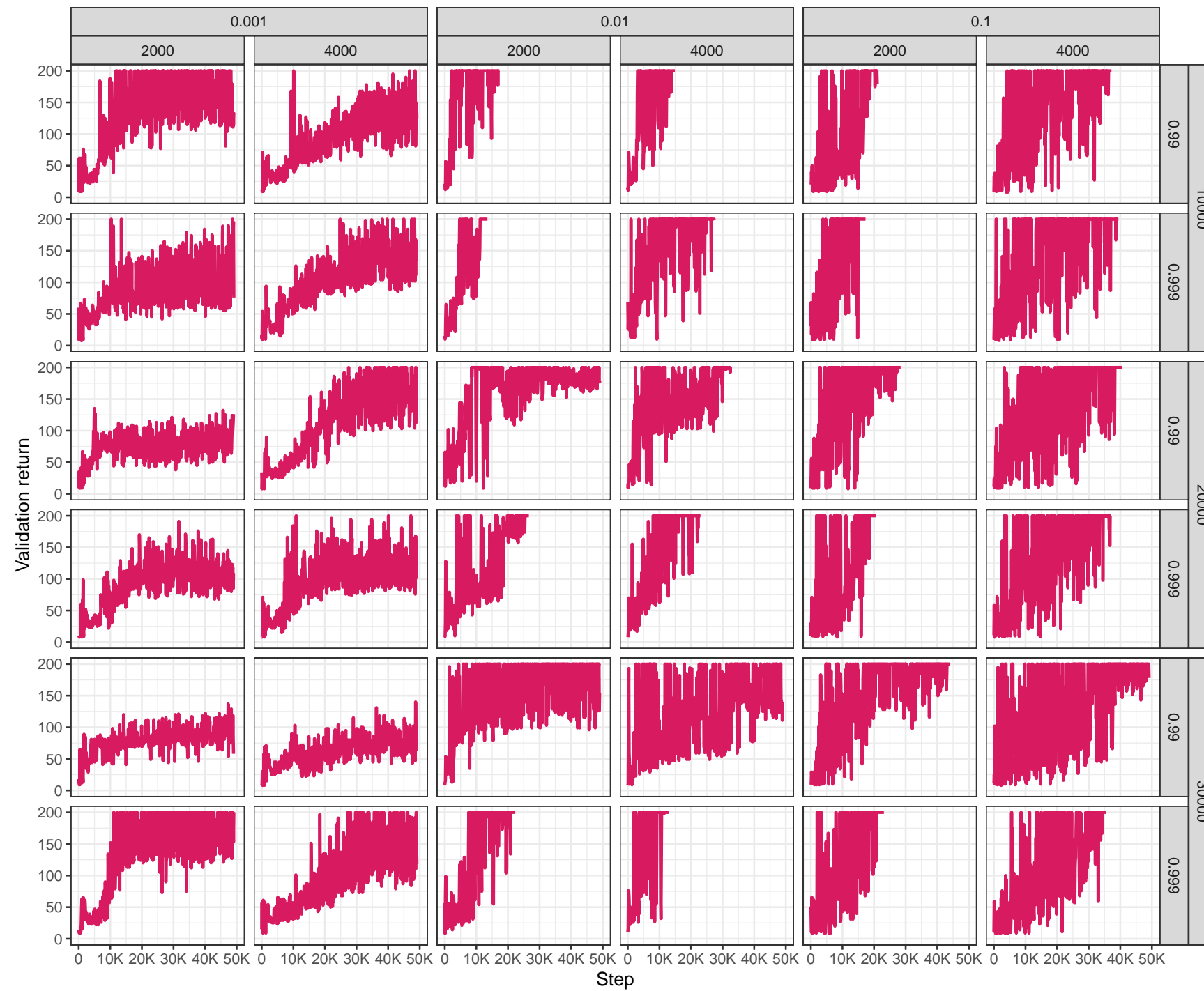
Data Re-Uploading – Skolik et al. – Global Scaling (GS) – Continuous (C)
