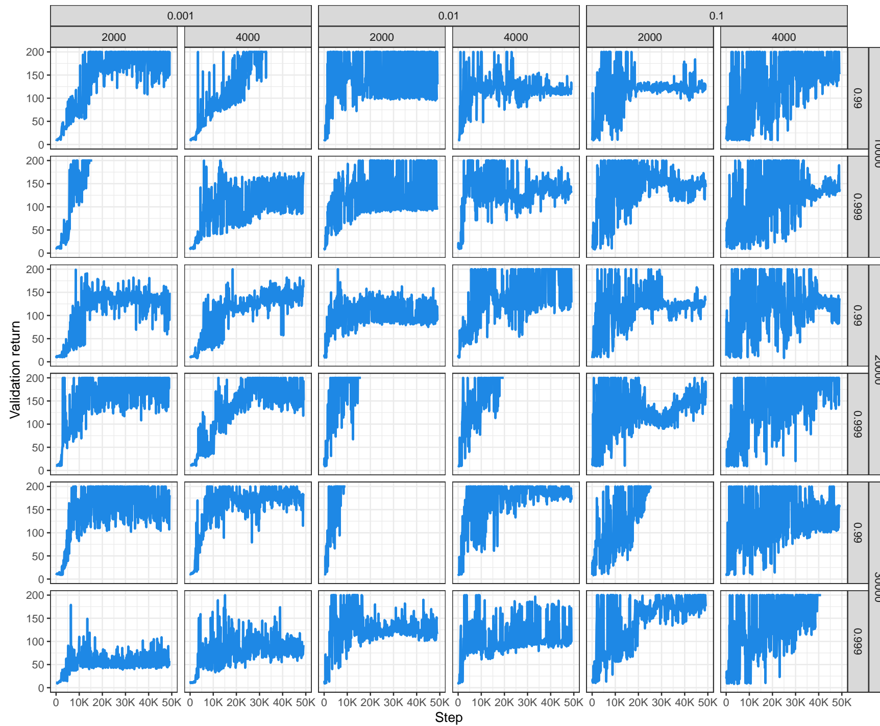
Data Re-Uploading – Lockwood and Si – Global Scaling with Pooling (GSP) – Scaled and Continuous (SC)
