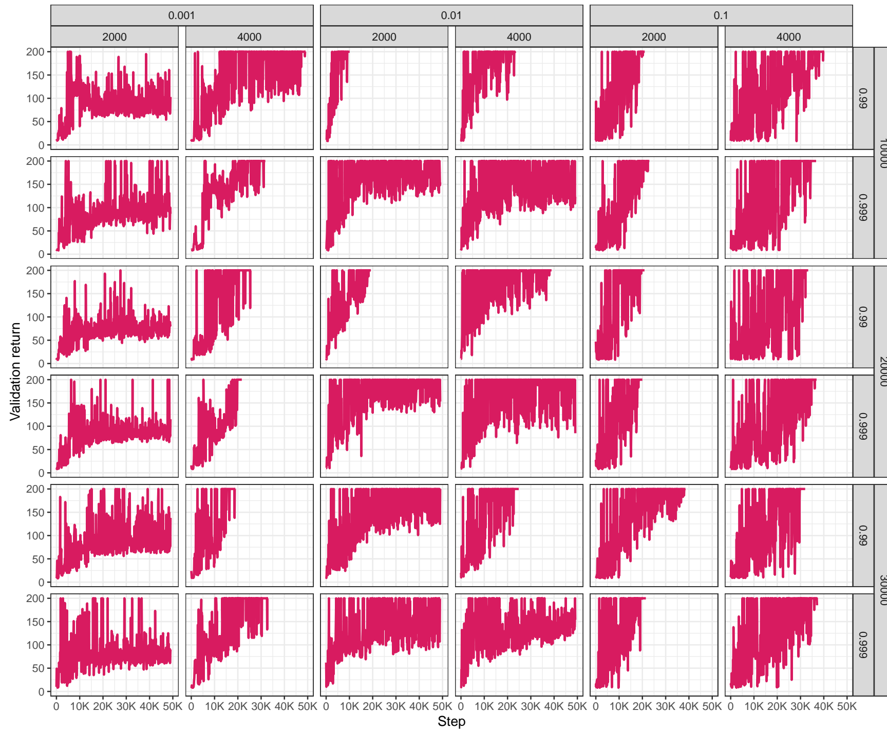
Data Re-Uploading – Lockwood and Si – Global Scaling with Pooling (GSP) – Continuous (C)
