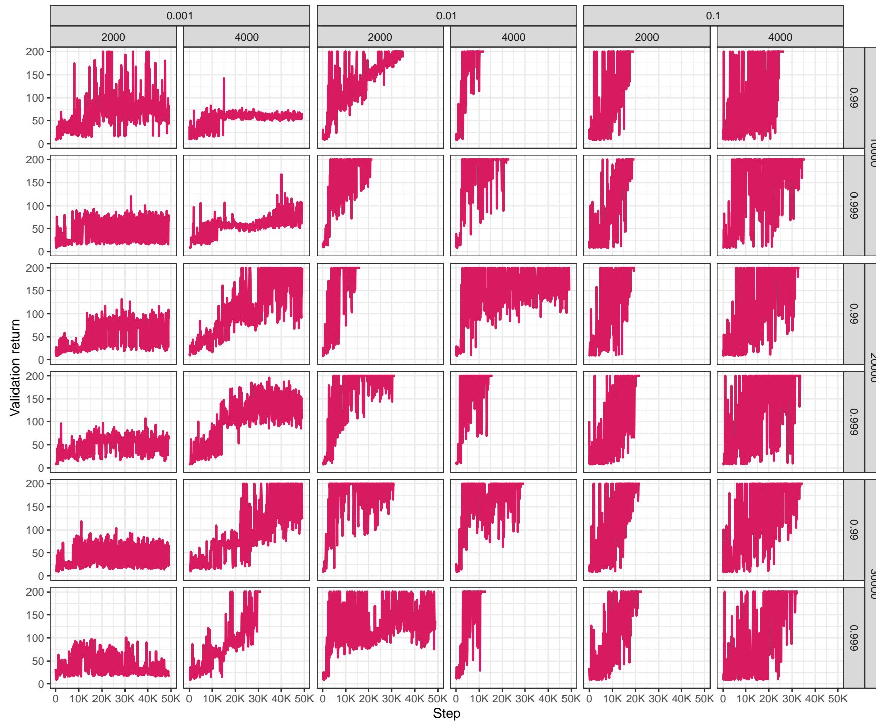
Data Re-Uploading – Lockwood and Si – Global Scaling (GS) – Continuous (C)
