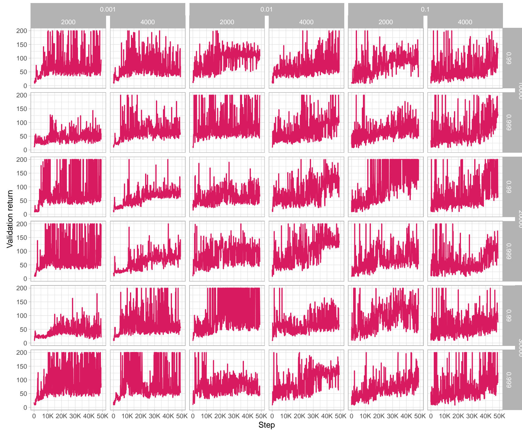
Skolik et al. – Global Scaling with Pooling (GSP) – Continuous (C)
