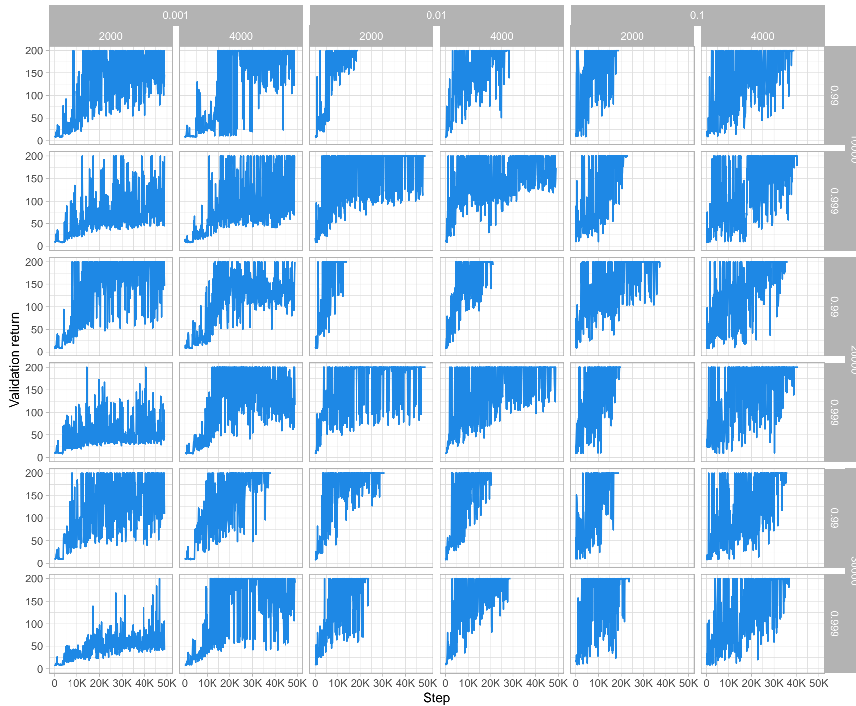
Lockwood and Si – Global Scaling with Pooling (GSP) – Scaled and Continuous (SC)
